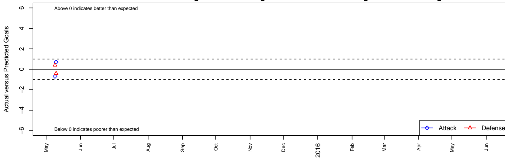
CB United Ephrata B00 Dots are actual minus expected GF (blue circles) and GA (red triangles). Blue line is smoothed change in attack strength. Red is smoothed change in defense strength.
